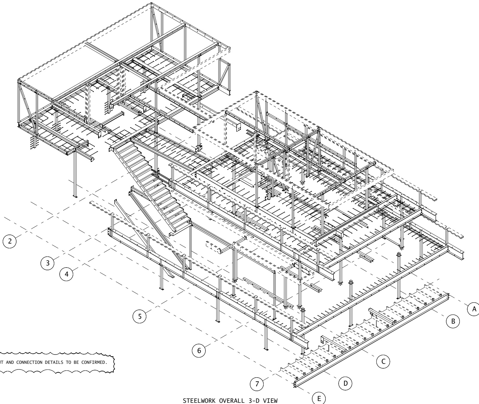
STEELWORK OVERALL 3-D VIEW
