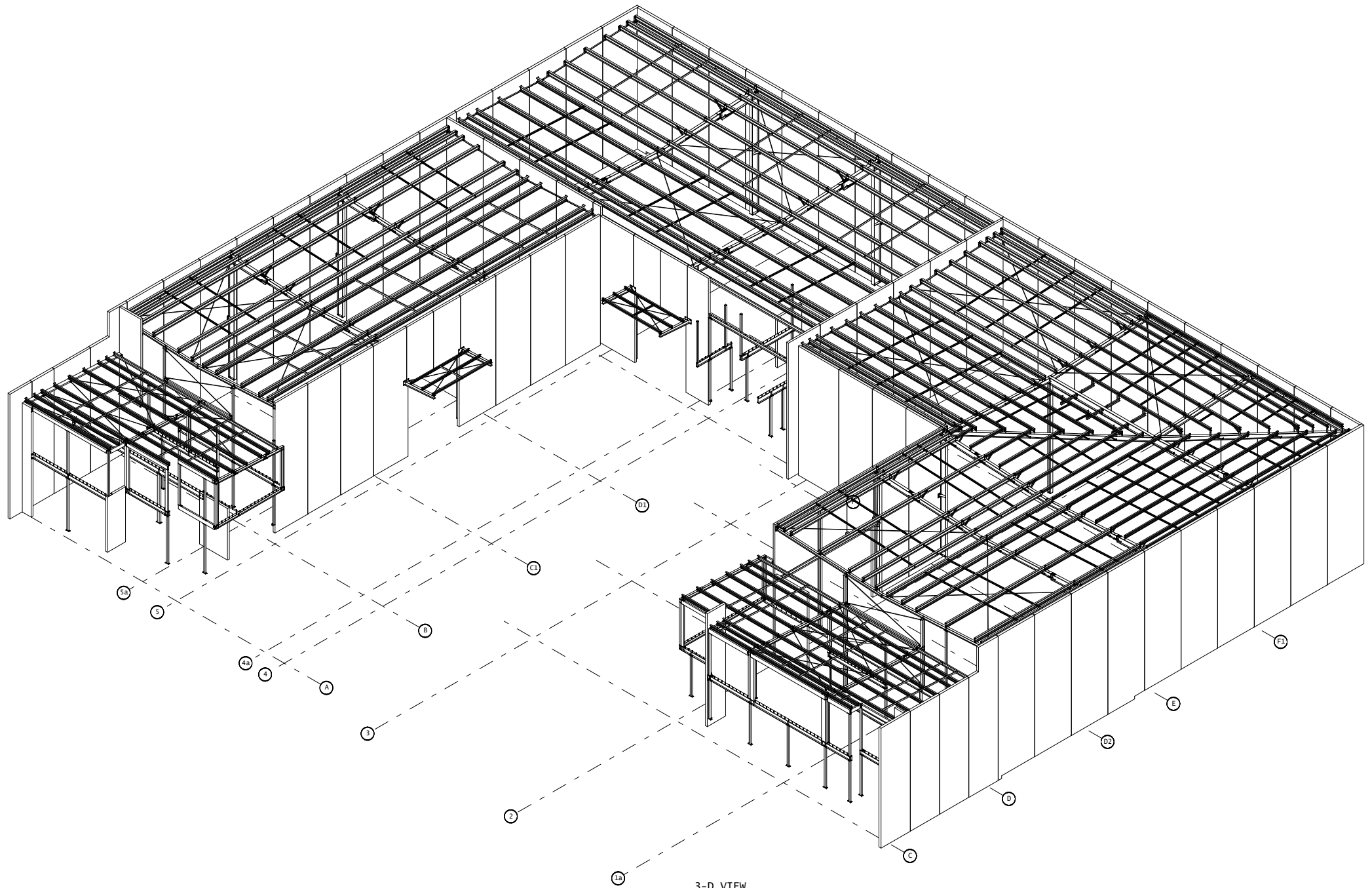
3-D VIEW
