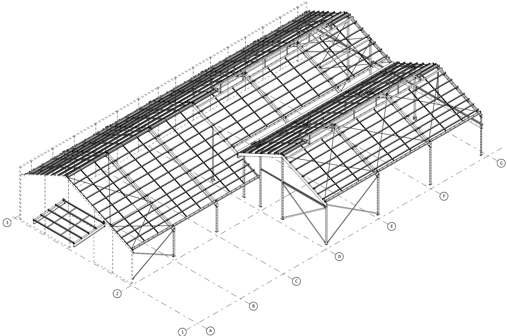
4 SQUARE OVERALL 3-D VIEW (2)
