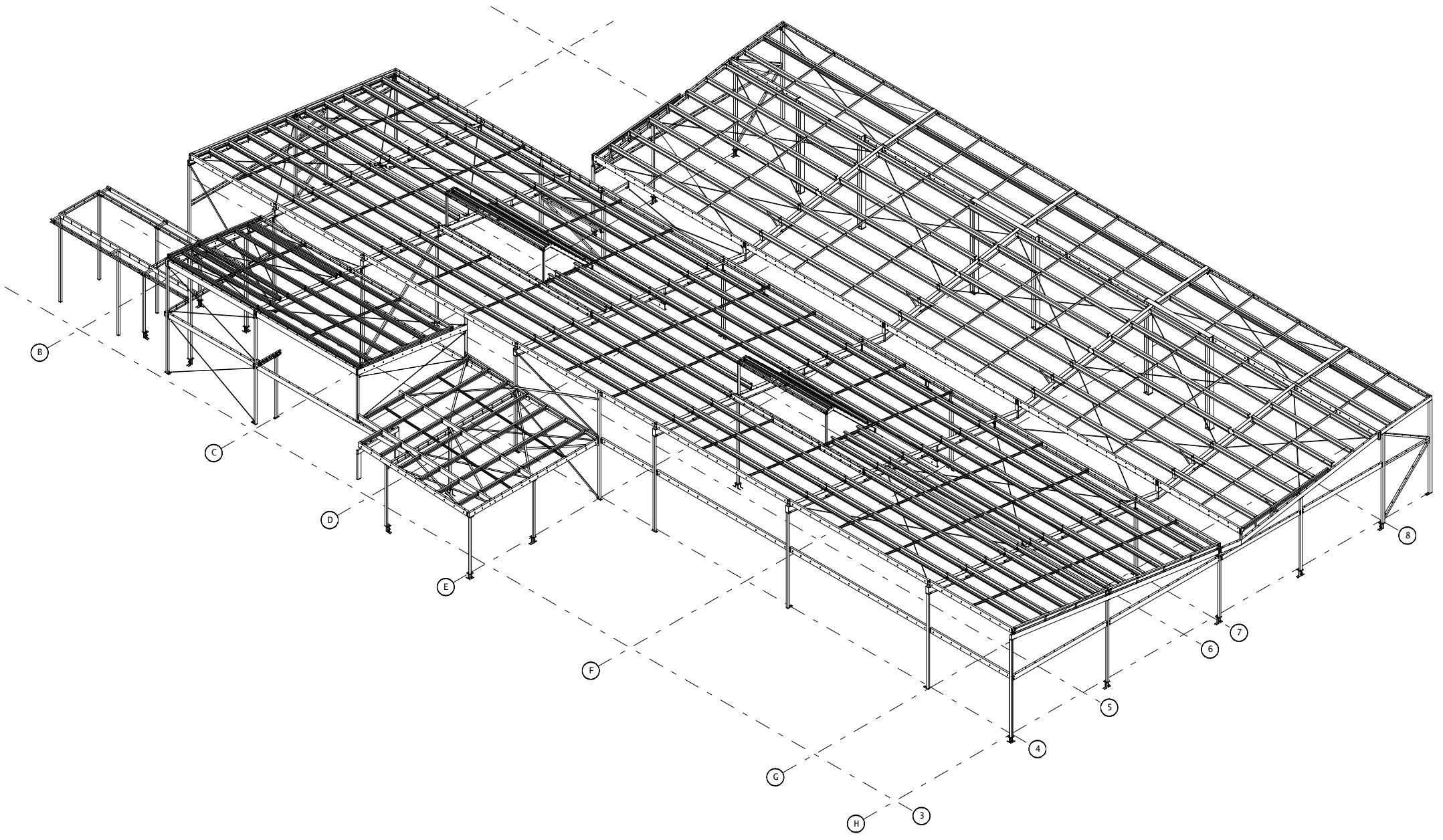
OVERALL 3-D VIEW (1)
