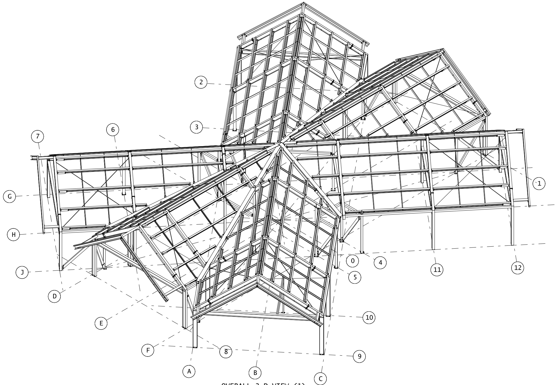
OVERALL 3-D VIEW (1)
