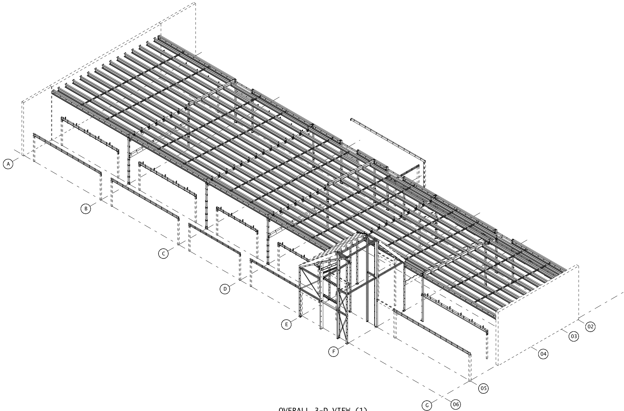
OVERALL 3-D VIEW (1)
