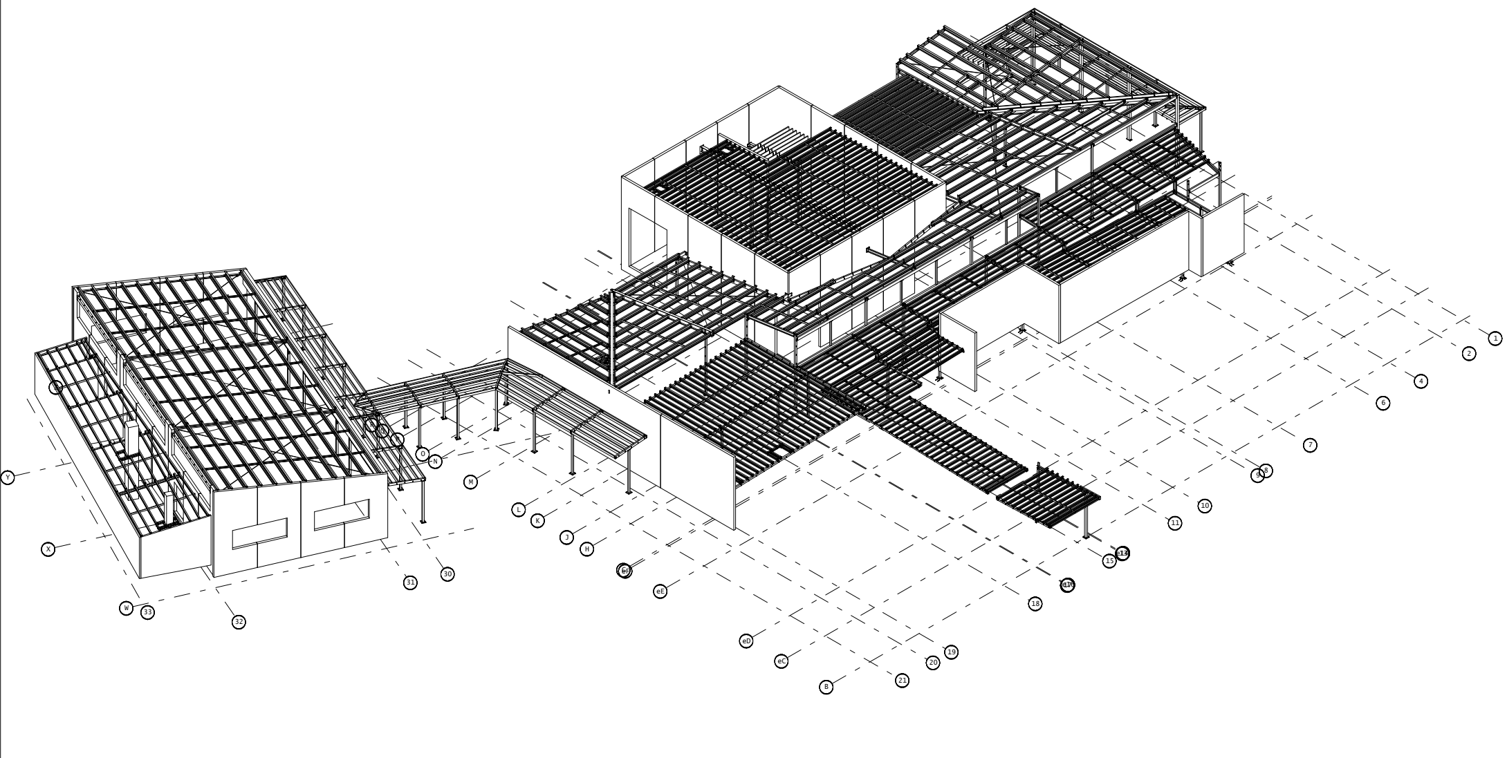
OVERALL 3-D VIEW
