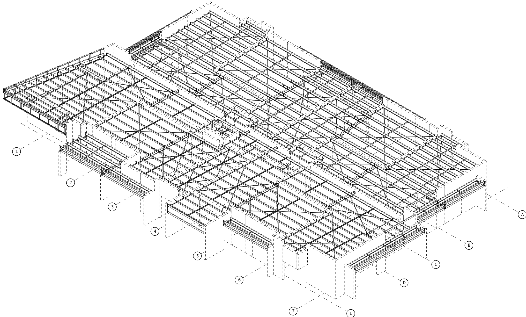
PHASE-3 OVERALL 3-D VIEW (1)
