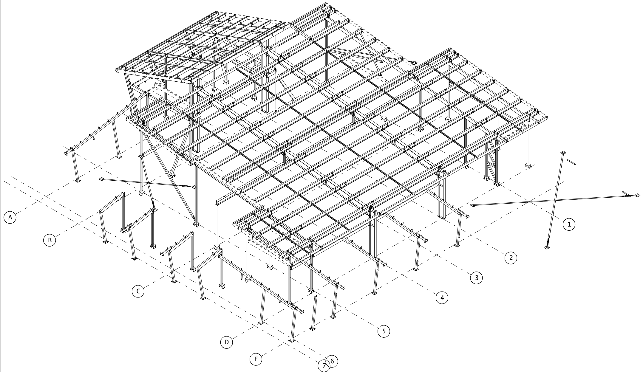
PHASE-1 OVERALL 3-D VIEW (1)
