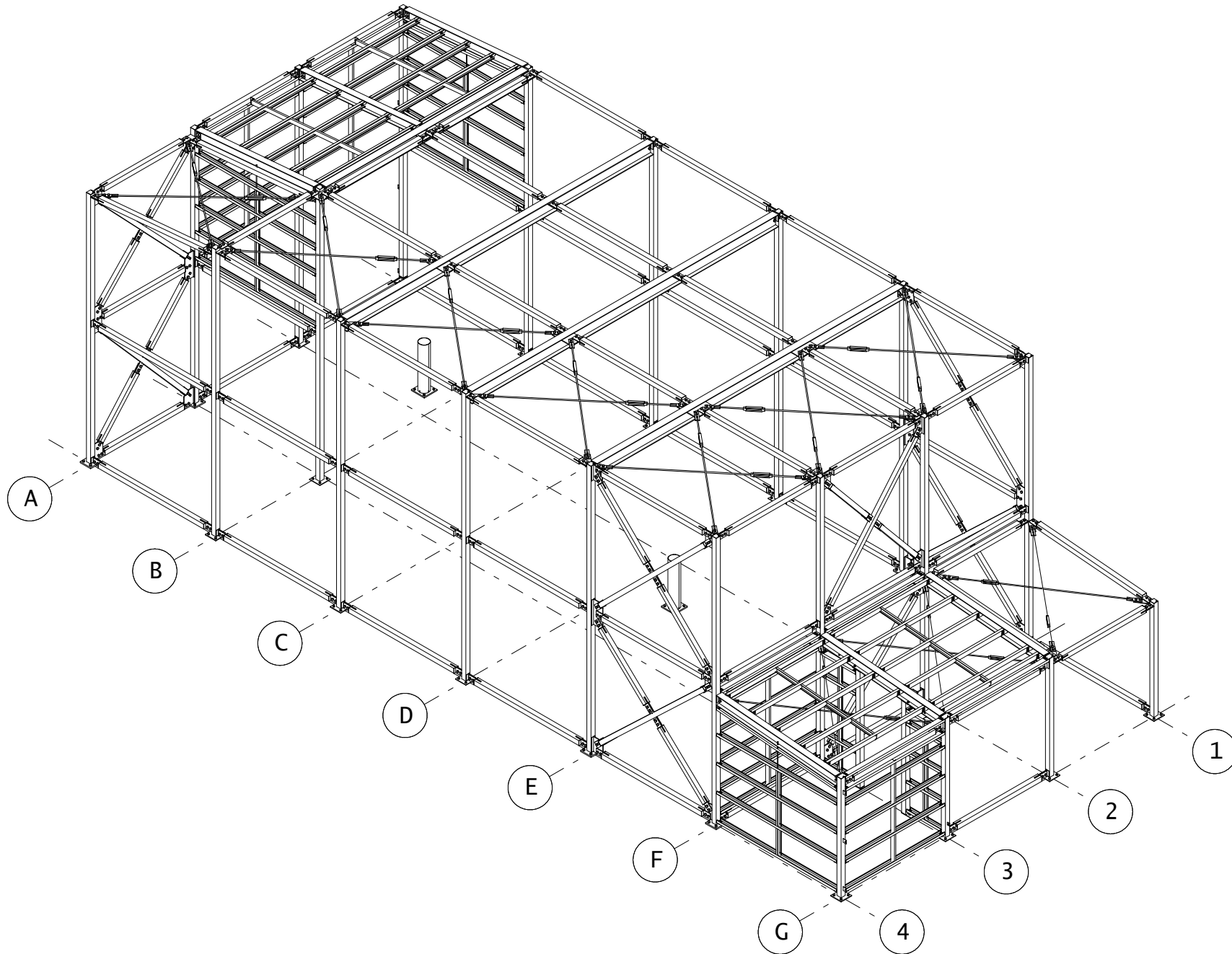
OVERALL 3-D VIEW (1)
